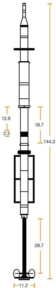
Tail Support Stand HALL P/N: AP1707-TSS-A-U
